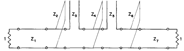
Fig. 4. Seven-section filter containing unit elements and stubs [6]. All sections are quarter-wave at 2.175 GHz.
